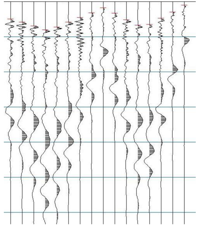
Figure 8. Raw waveform data from the Lilstock Beach experiment, showing the 16 geophone channels and the first arrival picks (red ticks). Onsets are clear and can be accurately picked.
