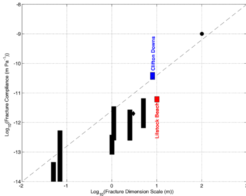
Figure 14. Compilation of measurements of fracture compliance as a function of fracture size. Modified from Verdon & Wüestefeld (2013).
